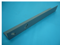
BRACKET 5K-LEFT L-65x65 LENGTH 500
