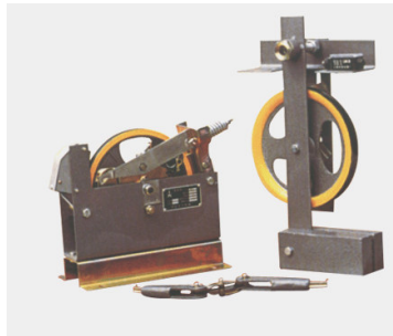
GOVERNOR WITH TENSION PULLEY SPEED 0.25 m/s, 0.5 m/s, 1.0 m/s 1.5 m/s, 1.75m/s
