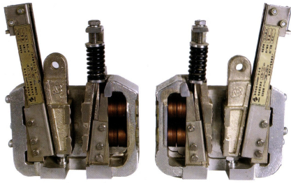
SAFETY GEAR QJ2500A MITSUBISHI TYPE RATED SPEED \leq 2.5 m/s
