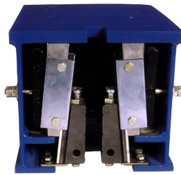
SAFETY GEAR QJ2500B HITACHI TYPE RATED SPEED \leq 2.5 m/s
