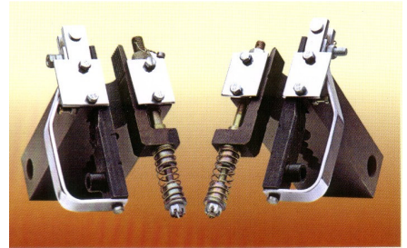
SAFETY GEAR AQ11 THYSSSEN TYPE RATED SPEED \leq 2.5 m/s
