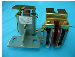
MITSUBISHI GUIDE SHOE 8K
