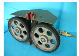
MITSUBISHI ROLLER GUIDE UNIT
