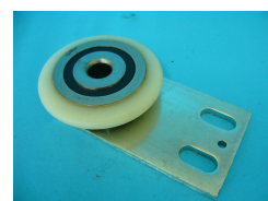
SCHINDLER HANGER ROLLER Ø75x12
