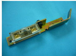
SCHINDLER QKS9 DOOR CONTACT-LEFT
